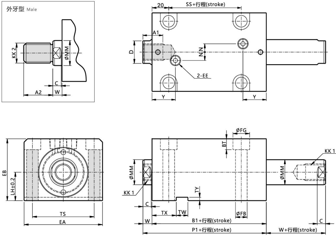
◆MPJ.Q.D 径向安装型双轴薄型油缸 Side mounting double stroke compact hydraulic cylinder
